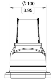
STANDARD MOUNTING CUTOUT
